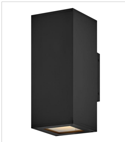
28914BK-LL SMALL WALL MOUNT LANTERN UP... 5" W, 12" H Socketed 2-7w GU10 LED *Included
