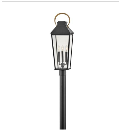
17501BK LARGE POST MOUNT LANTERN 9" W, 28.8" H Socketed 3-5w Cand. LED, 60w Equiv.
