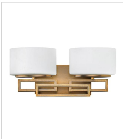
5102BR TWO LIGHT VANITY 16.3" W, 6.8" H Socketed 2-60w G-9 *Included or 2-5w G9 LED, 60w Equiv.
