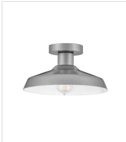
12072AL SMALL FLUSH MOUNT 12" W, 6.5" H Socketed 1-12w Med. LED, 100w Equiv.
