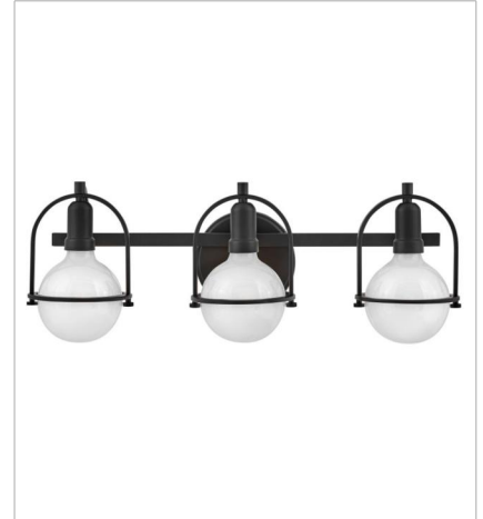
53773BK MEDIUM THREE LIGHT VANITY 25" W, 9" H Socketed 3-14w Med. LED, 100w Equiv.
