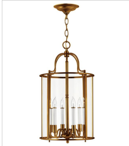
3478HR LARGE SINGLE TIER 14" W, 25" H Socketed 6-5w Cand. LED, 60w Equiv.
